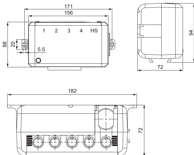
Outline drawing of corresponding controller of RD-F398
