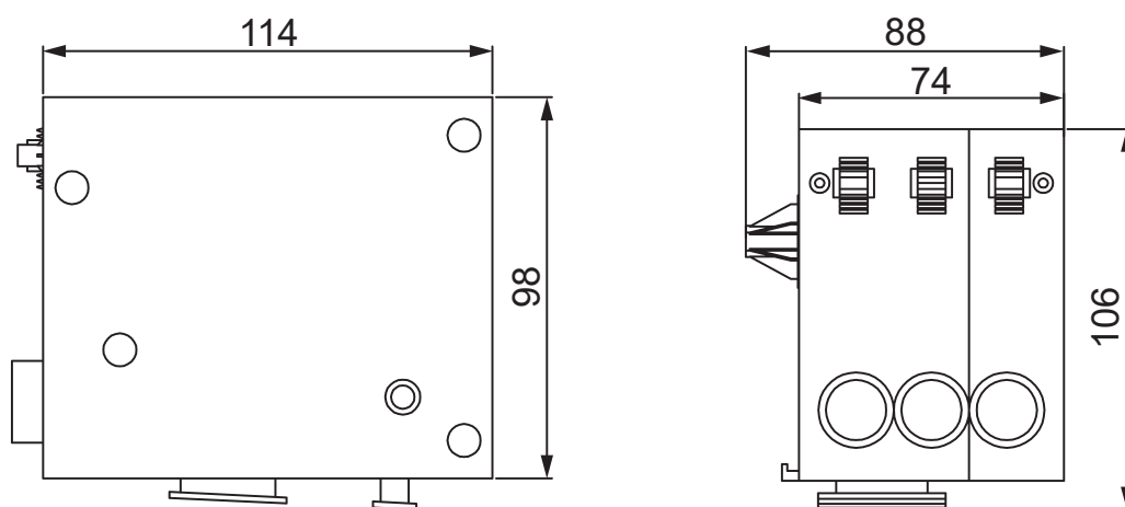
Outline drawing of corresponding controller of RD-A398
