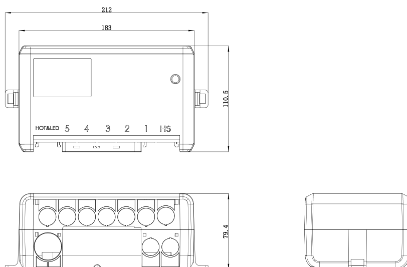
Outline drawing of corresponding controller of RD-H398
