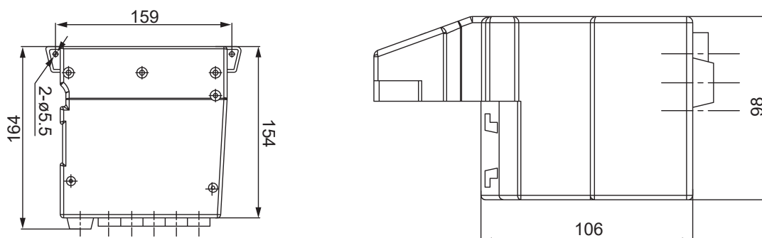
Outline drawing of corresponding controller of RD-D398
